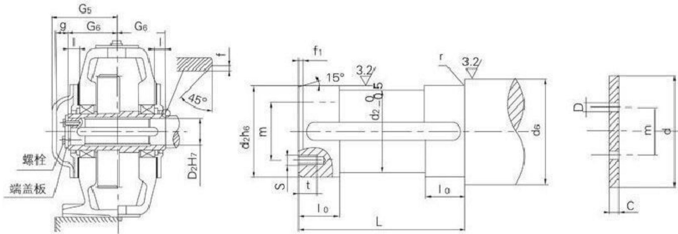
键槽按GB 1095-79
